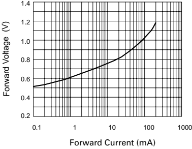
Forward Characteristics
